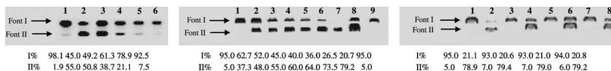
Figure 5. (a) Time-dependant photocleavage of DNA using C6 (100 μM). Lane 1: DNA alone (no hv); Lane 2: C6 and DNA (hv, 90 min); Lane 3: C6 and DNA (hv, 75 min); Lane 4: C6 and DNA (hv, 60 min); Lane 5: C6 and DNA (hv, 30 min); Lane 6: DNA alone (hv, 1.5 h). (b) Concentration-dependant photocleavage of DNA using C6 (hv, 1 h). Lane 1: DNA alone (no hv); Lane 2–8: DNA and C6 at concentrations of 2, 5, 10, 20, 50, 100, and 200 μM, respectively. Lane 9: DNA alone (hv). (c) pH effect on DNA photocleavage of C6 (100 μM; hv, 1 h). Lane 1, 3, 5, 7: DNA alone, pH = 8.5, 8.0, 7.5, 7.0, respectively; Lane 2, 4, 6, 8: DNA and C6, pH = 8.5, 8.0, 7.5, 7.0, respectively.
