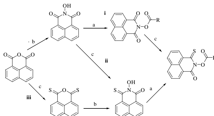
Scheme 2. Reagents and conditions: (a) \text{RCOCl} , \text{NEt}_3 , rt, 45 min; (b) \text{NH}_2\text{OH}\cdot\text{HCl} , \text{NEt}_3 , \text{CH}_3\text{CH} , reflux, 2 h; (c) Lawesson's reagent, \text{C}_6\text{H}_5\text{-Cl-}p , reflux, 1 h.
