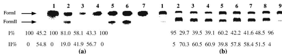
Figure 3. Photocleavage on pBR 322 DNA. The cleavage activities were evaluated using supercoiled circular pBR322 (form I) DNA (50 \mu M/bp) with the compound in the buffer Tris–HCl (pH 7.6) under photoirradiation (2300 \mu W/cm 2 ) with a transilluminator (366 nm) at a distance of 20 cm at 0 °C and then analyzed on a 1% agarose gel. DNA photocleavage efficiency was defined as the degree of relaxation of the supercoiled DNA, relaxed circular DNA (single-stranded cleavage) as form II. (a) Effects of different substituents on photocleavage (100 \mu M; hv, 45 min). Lane 1: DNA alone (no hv); Lane 2: DNA and C1 ; Lane 3: DNA and C2 ; Lane 4: DNA and C3 ; Lane 5: DNA and C4 ; Lane 6: DNA and C5 ; Lane 7: DNA alone (hv). (b) Effects of different substituents on photocleavage (100 \mu M; hv, 60 min). Lane 1: DNA alone (hv); Lane 2–8: DNA and C6 – C11 , C5 , respectively; Lane 9: DNA alone (no hv).
