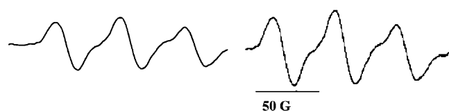
Figure 2. ESR spectroscopy of the radical released by C1 and C6 . ESR with PBN ( N-tert-butyl- \alpha -phenylnitrone ) trapping in benzene under light. Microwave frequency 9.782 GHz, mid range 3430 G, scan range.
