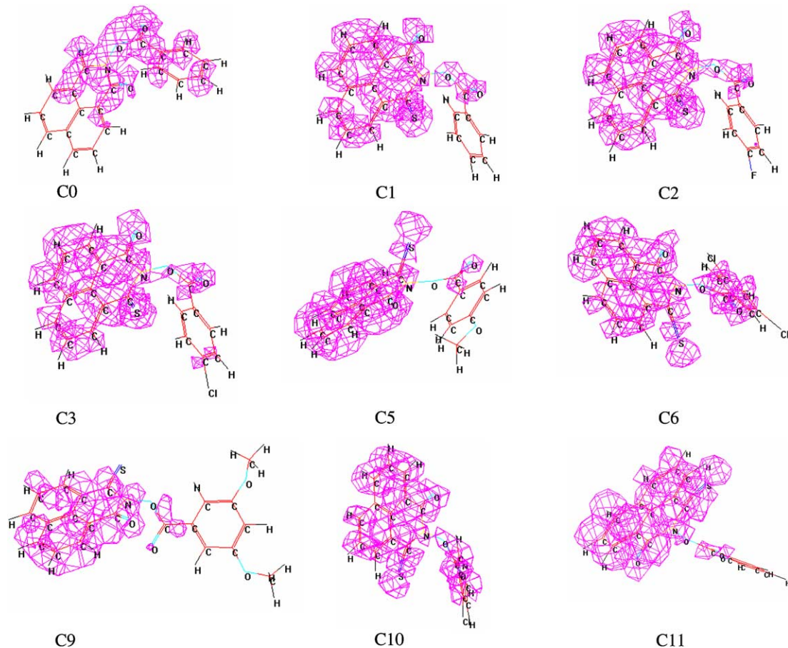
Figure 4. The distribution of electron clouds for the compounds.
